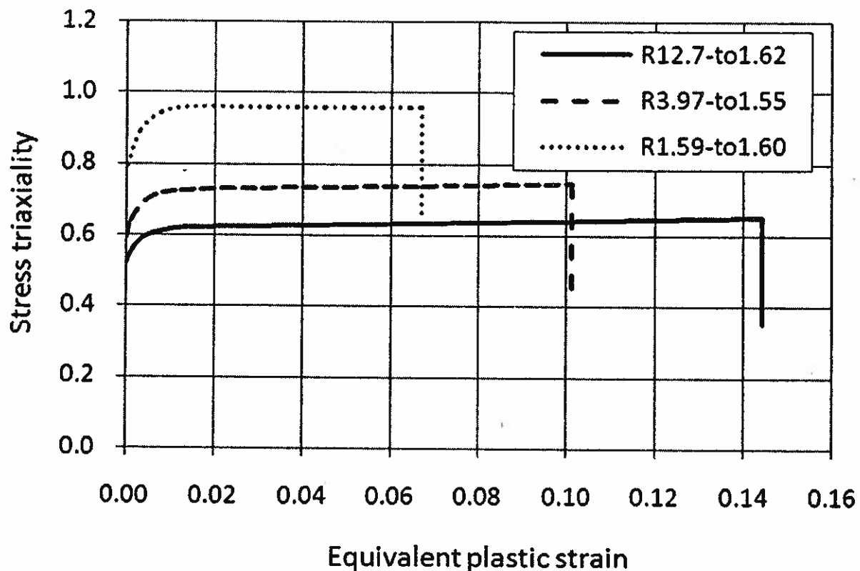
Figure 4: Stress Triaxiality Evolution Diagram of AISI Steel 1045 Obtained from Finite Element Simulation for three Selected Flat-Grooved Specimens
