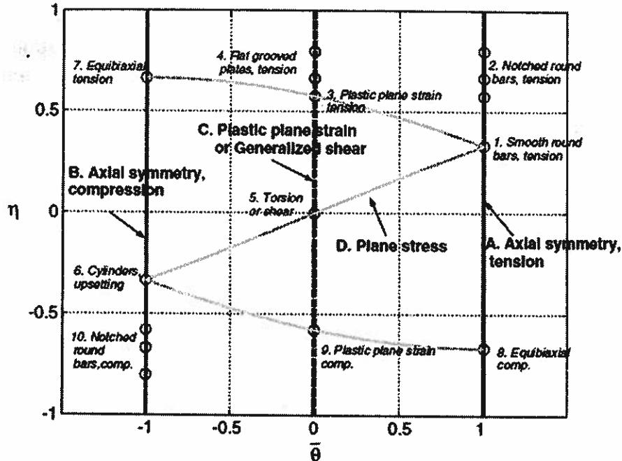
Figure 2: Stress States Diagram in the Triaxiality and Lode Angle Parameter (Equivalent to \xi ) [15]
