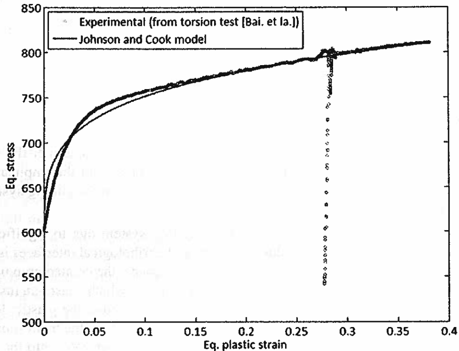
Figure 1: JC Equivalent Plastic Flow Model Optimization for AISI Steel 1045 Based on Torsion Test Performed by Bai. et al.[1]
