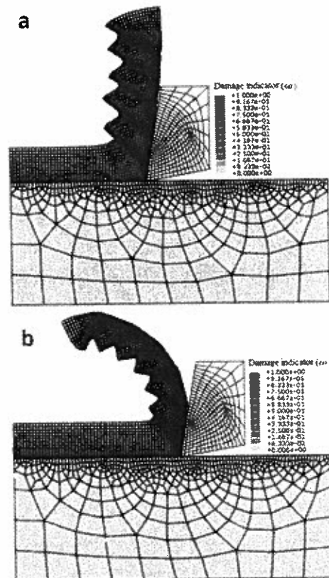
Figure 9: Finite Element Simulation of the Serrated Chip Formation with: (a) Contact Friction, and (b) No Friction at the Tool-Chip Interface
