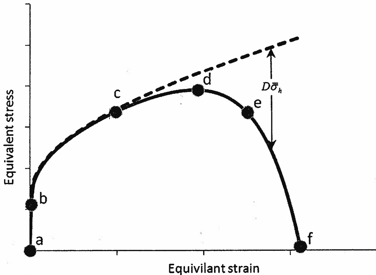
Figure 7: Typical Metal Stress Strain Response in a Uniaxial Test
