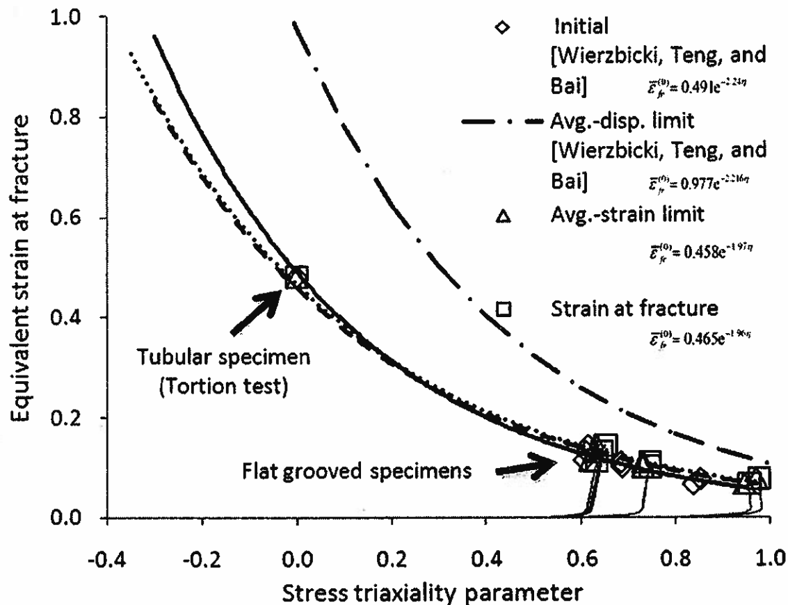
Figure 5: AISI Steel 1045 Fracture Locus Based on Initial Stress Triaxiality, Averaged using Displacement Limit Simulation Model, Averaged using Strain Limit Model, and the Fracture Locus Based on Strain at Fracture. Stress Triaxiality Evolution Curves are Also Shown
