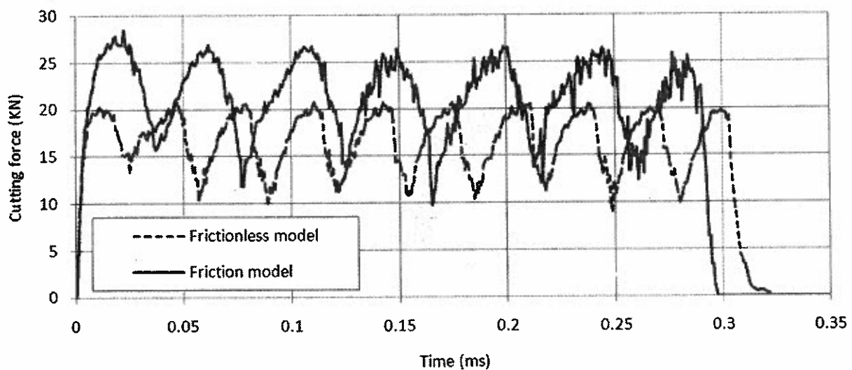
Figure 11. Cyclic of the Cutting Forces for Machining AISI Steel 1045 with and Without Accounting for Tool-Chip Interface Friction
