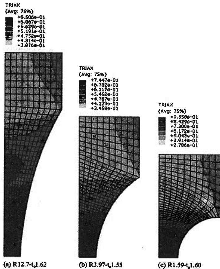
Figure 3: Axis-Symmetric Finite Element Simulation with the Stress Triaxiality Contours at Fracture for three Selected Flat-Grooved Specimens Made of AISI Steel 1045. Specimen (a) Groove radius R = 12.7 mm, Ligament Thickness t_0 = 1.62 mm, Specimen (b) R = 3.97 mm, t_0 = 1.55 mm, and Specimen (c) R = 1.59 mm, t_0 = 1.60 mm
