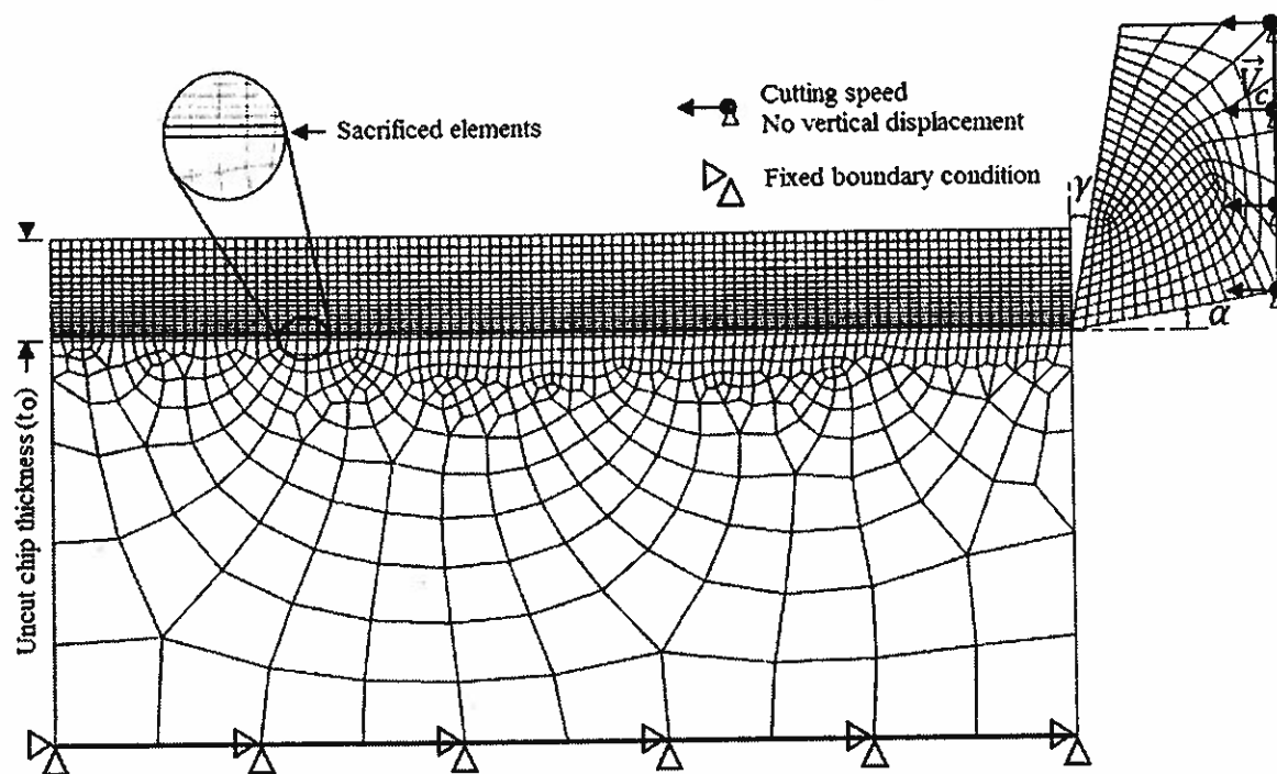
Figure 8: Finite Element Model: the Undeformed Mesh and the Prescribed Boundary Condition
