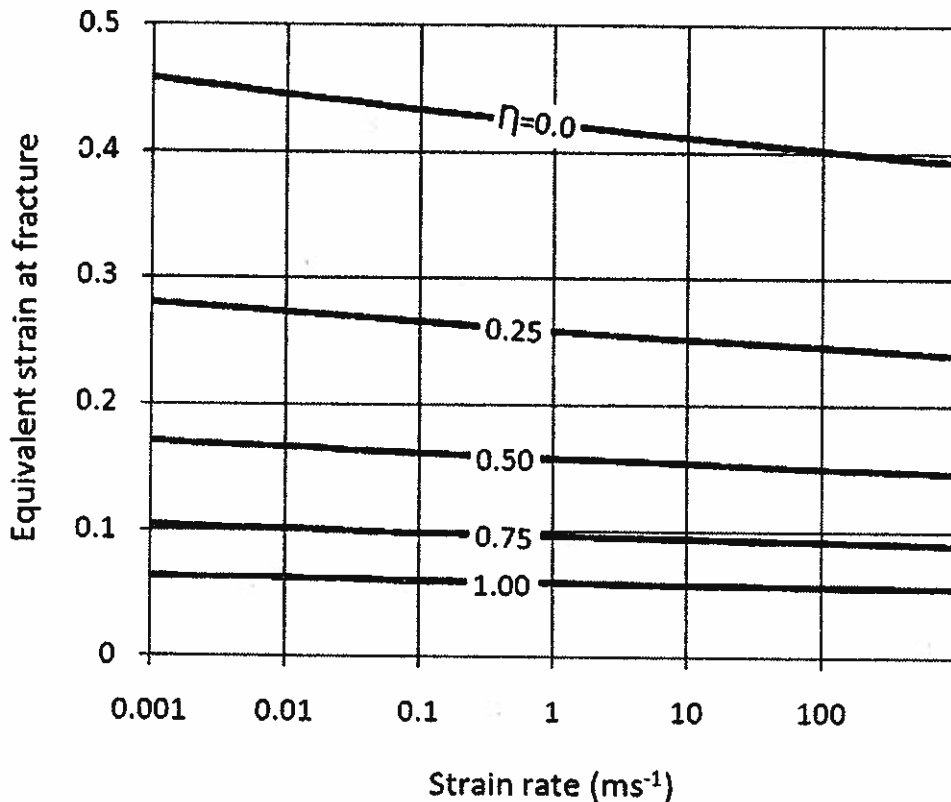
Figure 6: The Strain Rate Impact on the Equivalent Fracture Strain at Different Stress States for AISI Steel 1045
